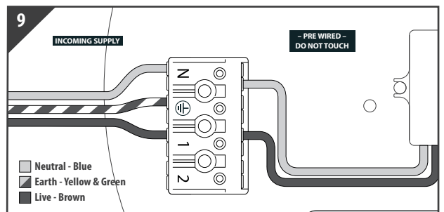
9 Press the individual terminal and insert the correct incoming supply before releasing the terminal to secure. The product MUST be earthed
