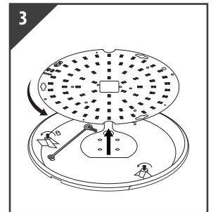
3 Loosen screws and twist to remove gear tray from the base, detach safety belt
