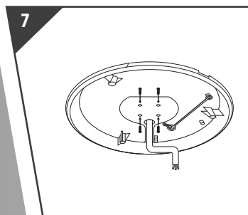
7 Install the fixing screws to the base plate
