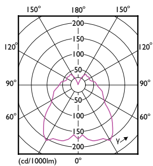
LEDcandle MAS SLR1 B38 5,5W B15 827 CL-LDD
