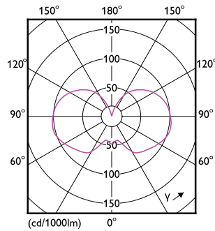
Light Distribution Diagram - MAS LEDBulbDT5.9-60WB22 927A60CL G UK
