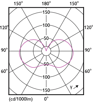
Light Distribution Diagram - MAS LEDBulbDT3.4-40WB22 927A60CL G UK
