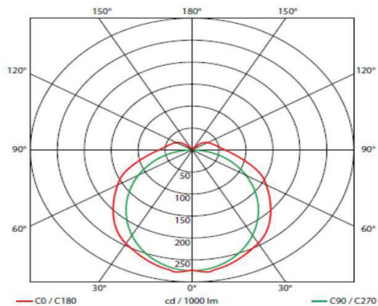
Light distribution diagram
