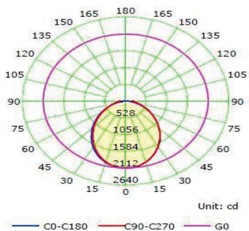
Light distribution diagram
