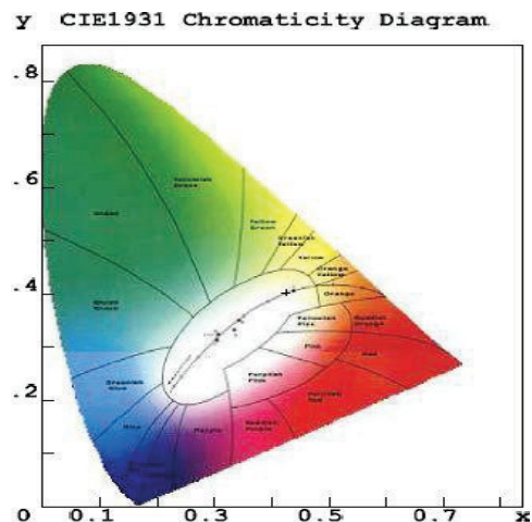
Chromaticity plot
