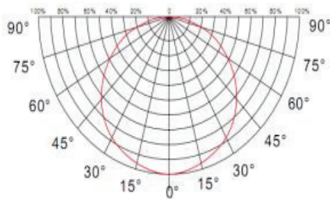
Relative luminous intensity lv % LED Light distribution
